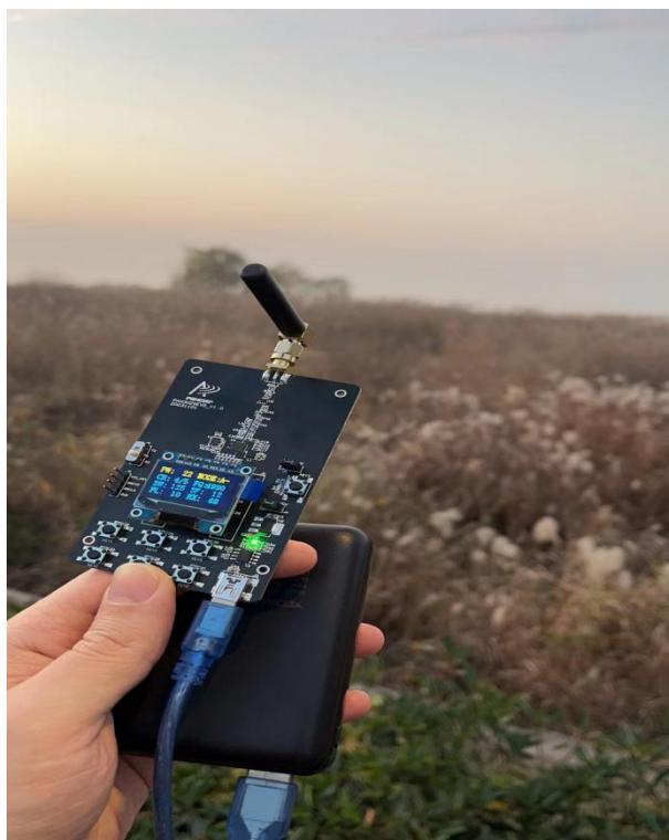
Figure 3-52 Receiver environment at a distance of 20,230 meters
